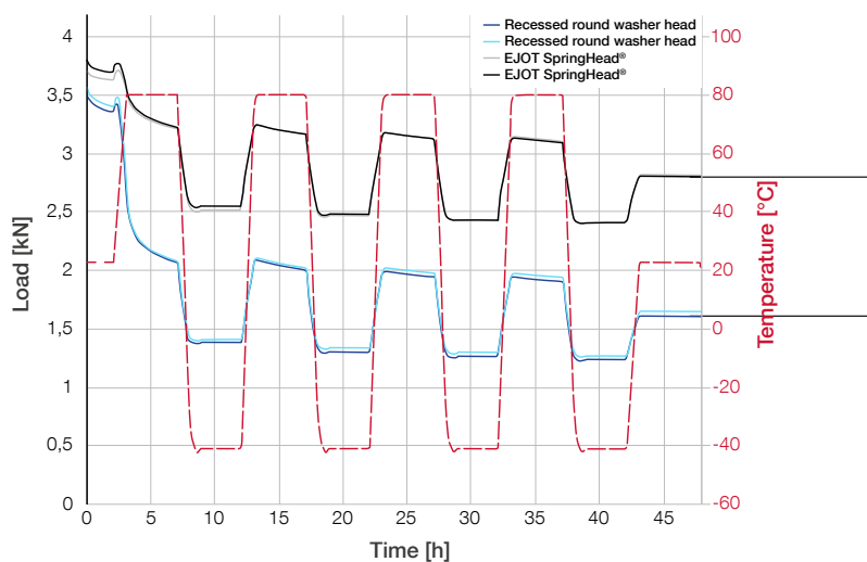
Comparison of clamp load relaxation: Recessed round washer head vs. EJOT SpringHead®
